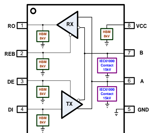
Functional Block of AZRS7032P
