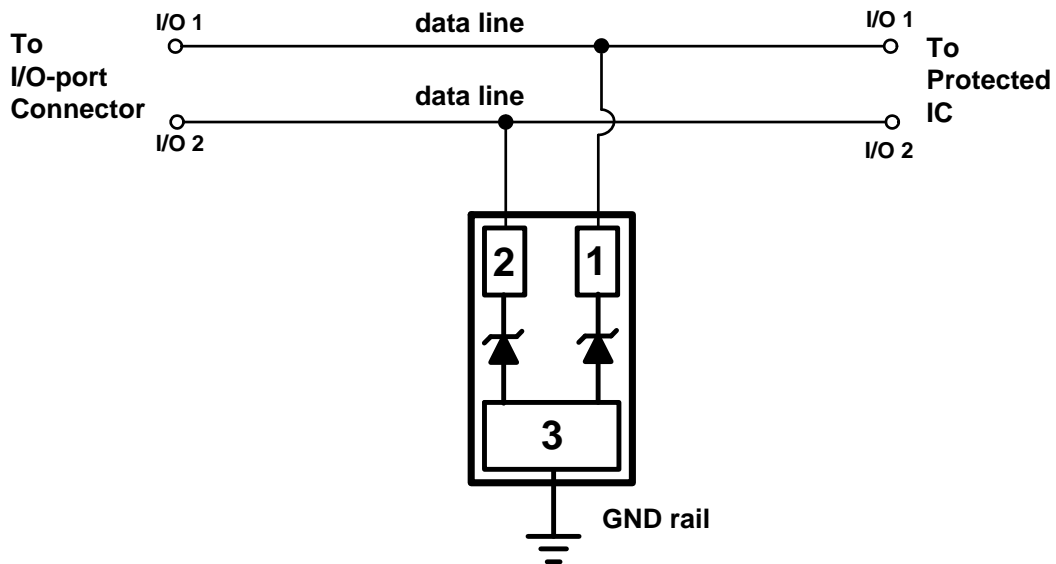
Fig. 1 Data lines connection of AZ9515-02F.
