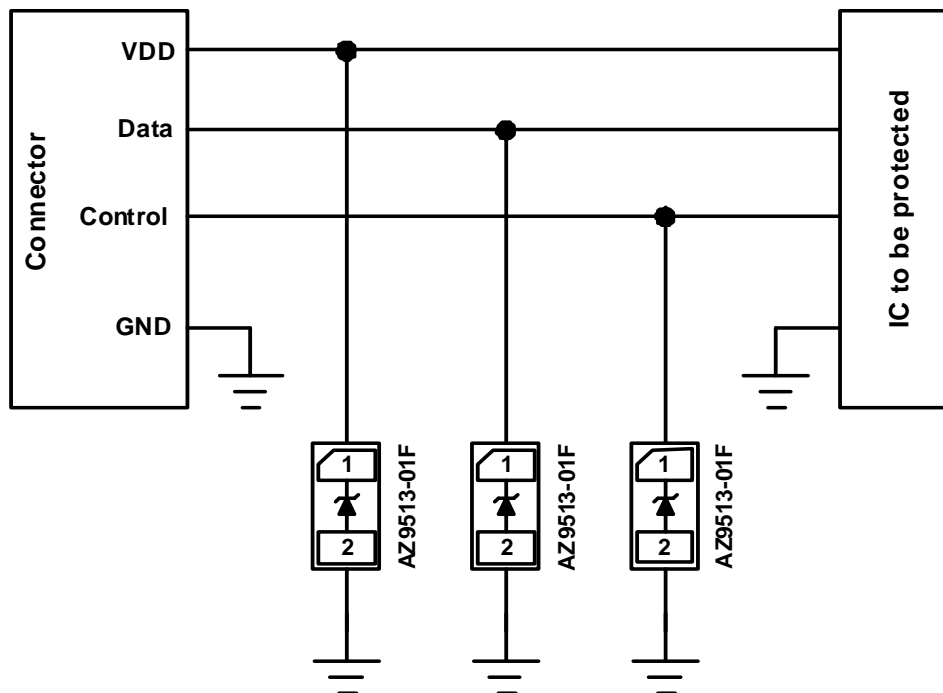
Fig. 1 ESD protection scheme by using AZ9513-01F.
