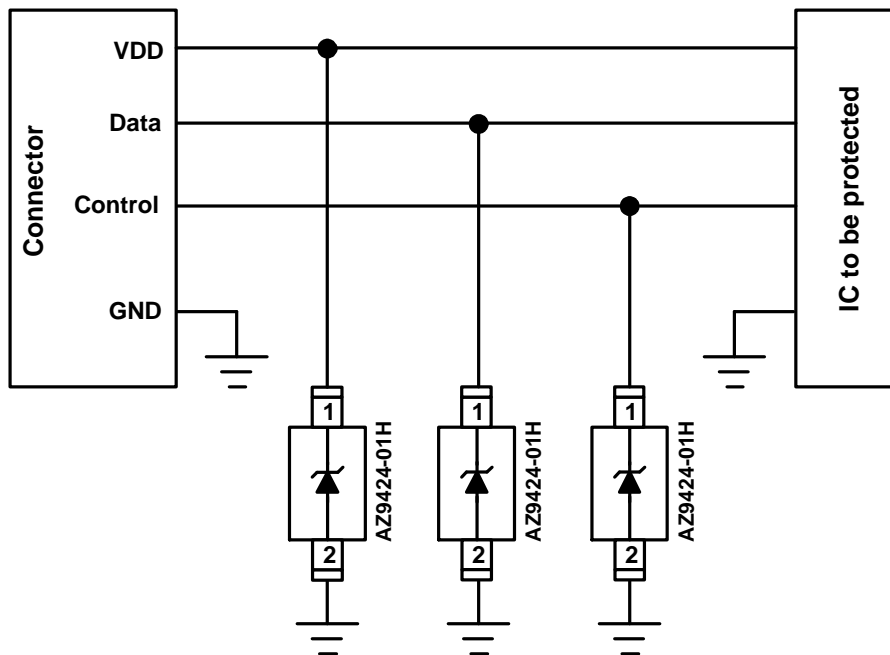
Fig. 1 ESD protection scheme by using AZ9424-01H.
