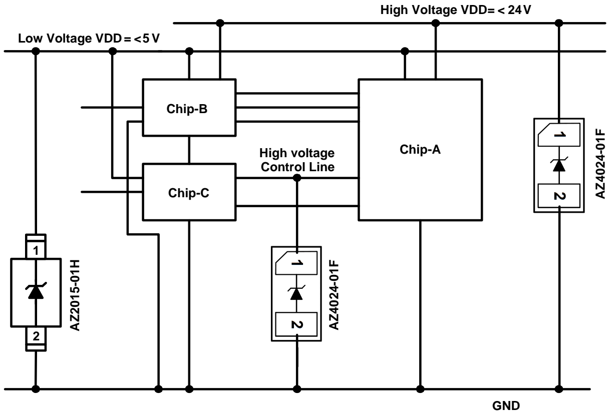
Fig. 1 ESD protection scheme for internal PCB circuits by using AZ4024-01F.
